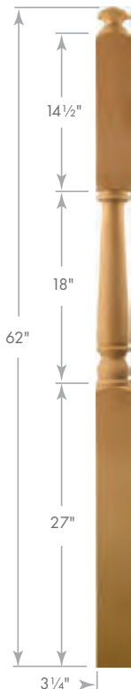
INTERMEDIATE LANDING B3186 (4186-MT)
