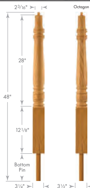
Plain B3294C Octagon B3294C-O
