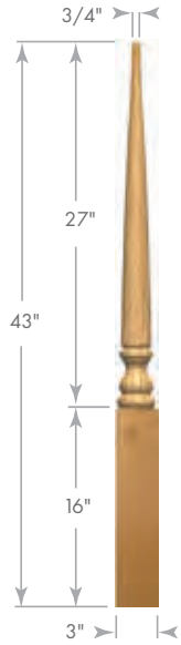
Rake Newel STARTING B320-PIN (4013)
