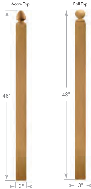
Acorn Top STARTING B3242-AC
