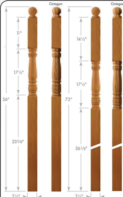
Plain B3293 (4503-BT) Octagon B3293-O (4503-BT-OCT) Plain B3295 (4505-BT) Octagon B3295-O (4505-BT-OCT)
