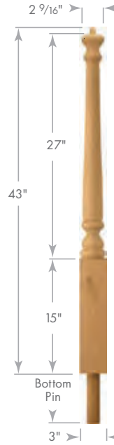
VOLUTE/TURNOUT (Adjustable) B3221C
