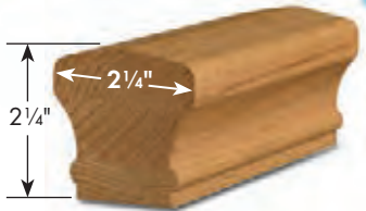
B5000 (C6601) Available Plowed for 1 1/4"
