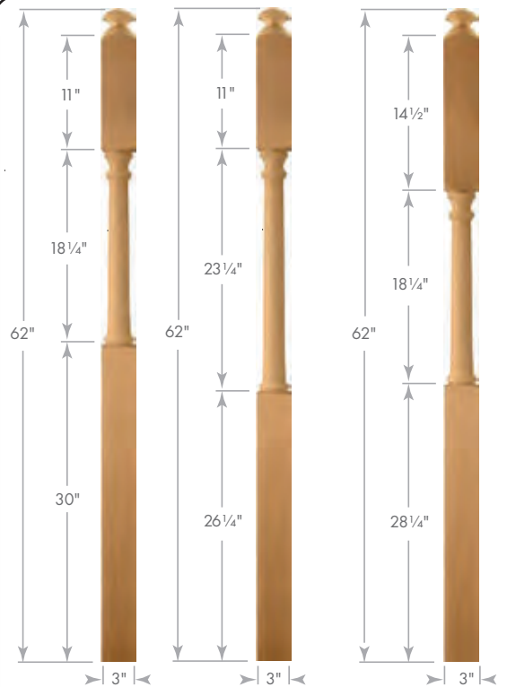
Mushroom Top 2ND FLOOR B3244
