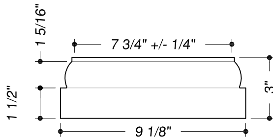
Base
