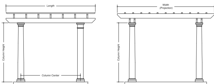
Front View Beam / Structural rafters run the length of the pergola.
