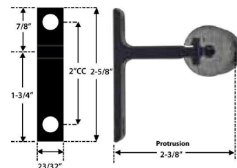
Long Bracket
