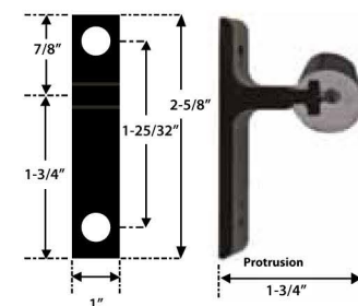
Short Bracket
