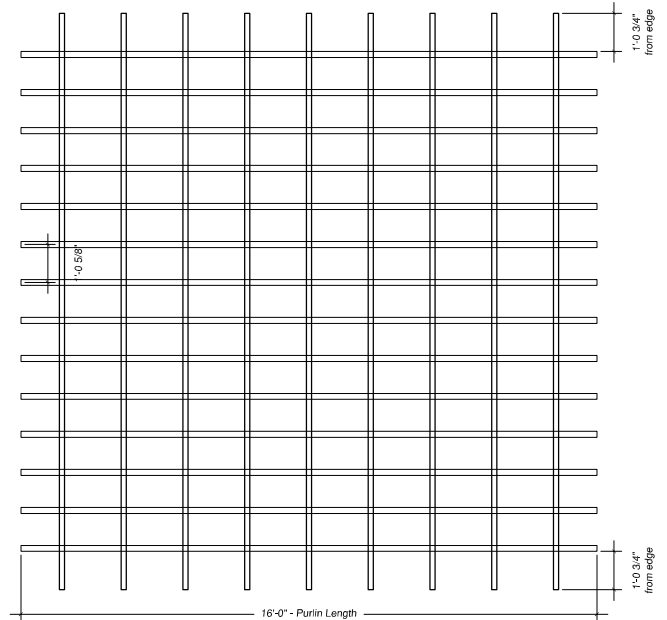
Purlins and Rafters
