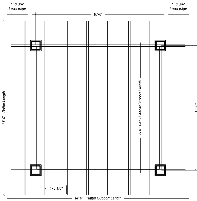
Rafters and Rafter Supports
