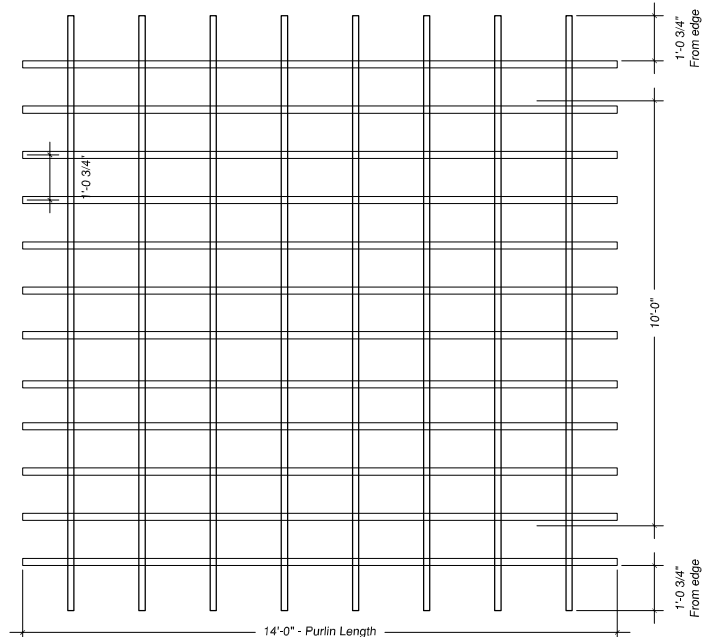
Purlins and Rafters
